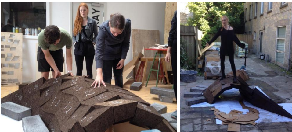
Figure 2: (Left) Students test strength of vault (Right) Standing on the vault to test its strength.
