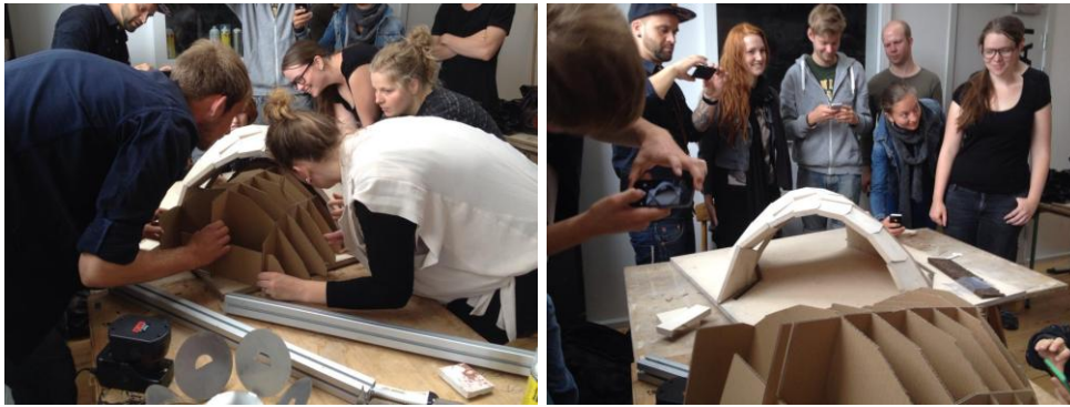
Figure 1: (Left) Centering being removed from the plywood vault. (Right) Free-standing plywood test vault with centering in foreground.
