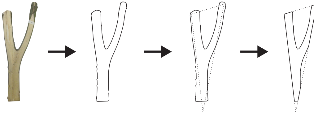
Figure 8 'Triangulated Branches' explored the potentials within using branches as elements in a triangulated polygonal surface through registering each Y-Shaped branch by its bounding-box fitting in a triangle of the controlled po- lygonal surface. Each branch was further processed and flattened with two parallel surfaces for making it more convenient to work with in standard wood-shop machin- ery (A Brunvoll, A Bergqvist, A Schumann, M Bhuvanendra).
