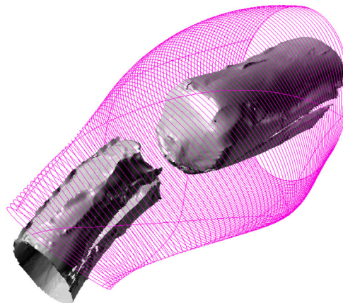
Figure 2 'Prosthetic Branching' created experimental joints whose functions were to form the merging pieces between a pair of branches. A detailed scan of the end of the crotches served as the negative for the interior shape of a clamp encompassing the whole end of the branch. The joint were milled in MDF on a 3-axis-router. (L K Madsen, V A Velarde, H Martinez, M Giodice)
