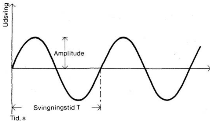
Figure 2. Sound is often pictured as a wave. The distance between the waves indicates the frequency, while the wave height indicates how loud the sound is (Petersen, 1984).
