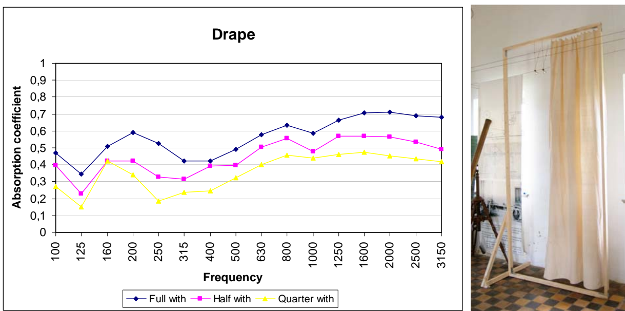
Figure 4. The graph shows the importance of the draping of the textile. The photo shows one of the two frames with textile.
