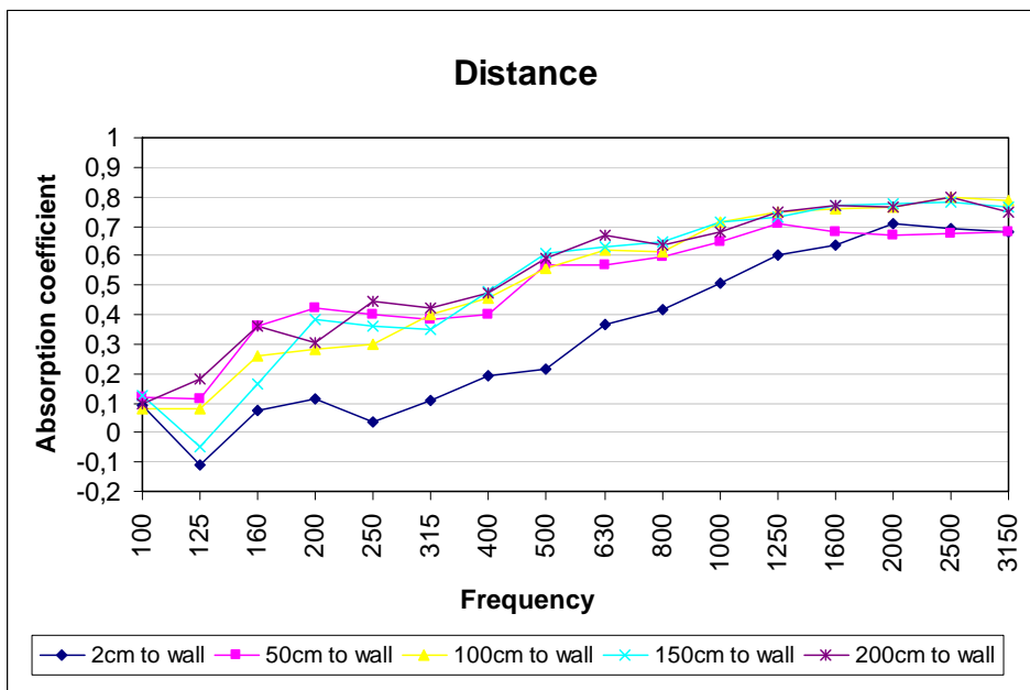
Figure 3. The graph shows the importance of the distance from the textile to the wall. The photo shows one of the two frames with textile.
